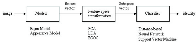
Figure 1: The procedure and some popular methods for face recognition/verification
